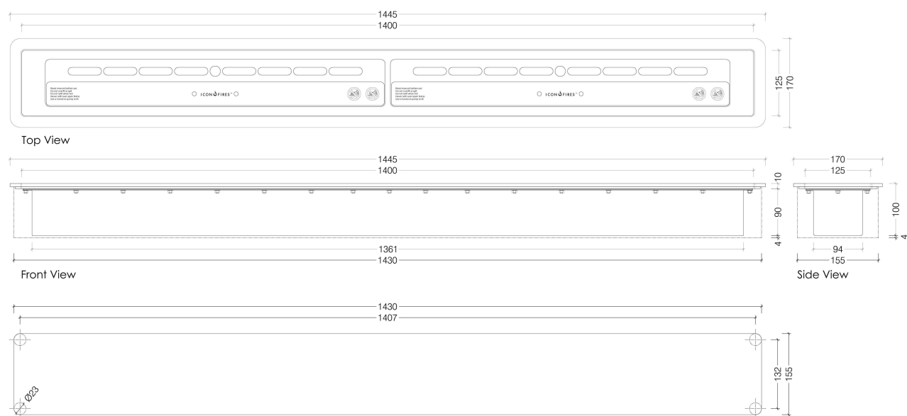
Slimline 1400 Biofuel Burner With Mount Plate
