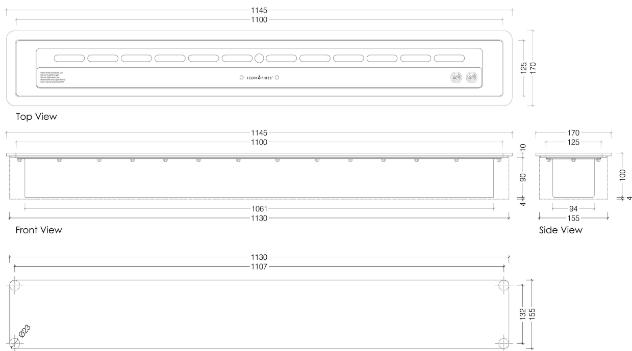
Slimline 1100 Biofuel Burner With Mount Plate
