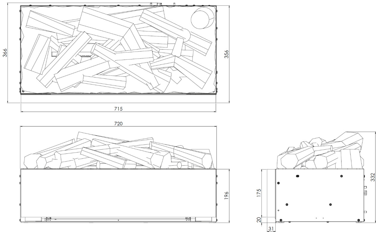
Dimensional Drawing Juneau XL multi
