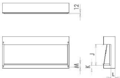
Shown with both side panel removed to give greater design opportunities of installation
