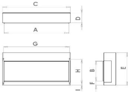
Shown as supplied for front opening arrangement with side panels in position either or both side panels can be removed to give a 2 sided or 3 sided arrangement
